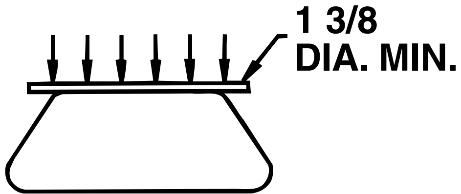
Spread Load Drawing
